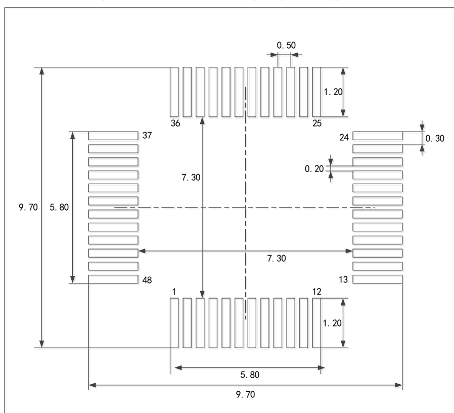
Figure 18 LQFP48 Welding Layout Suggestion
