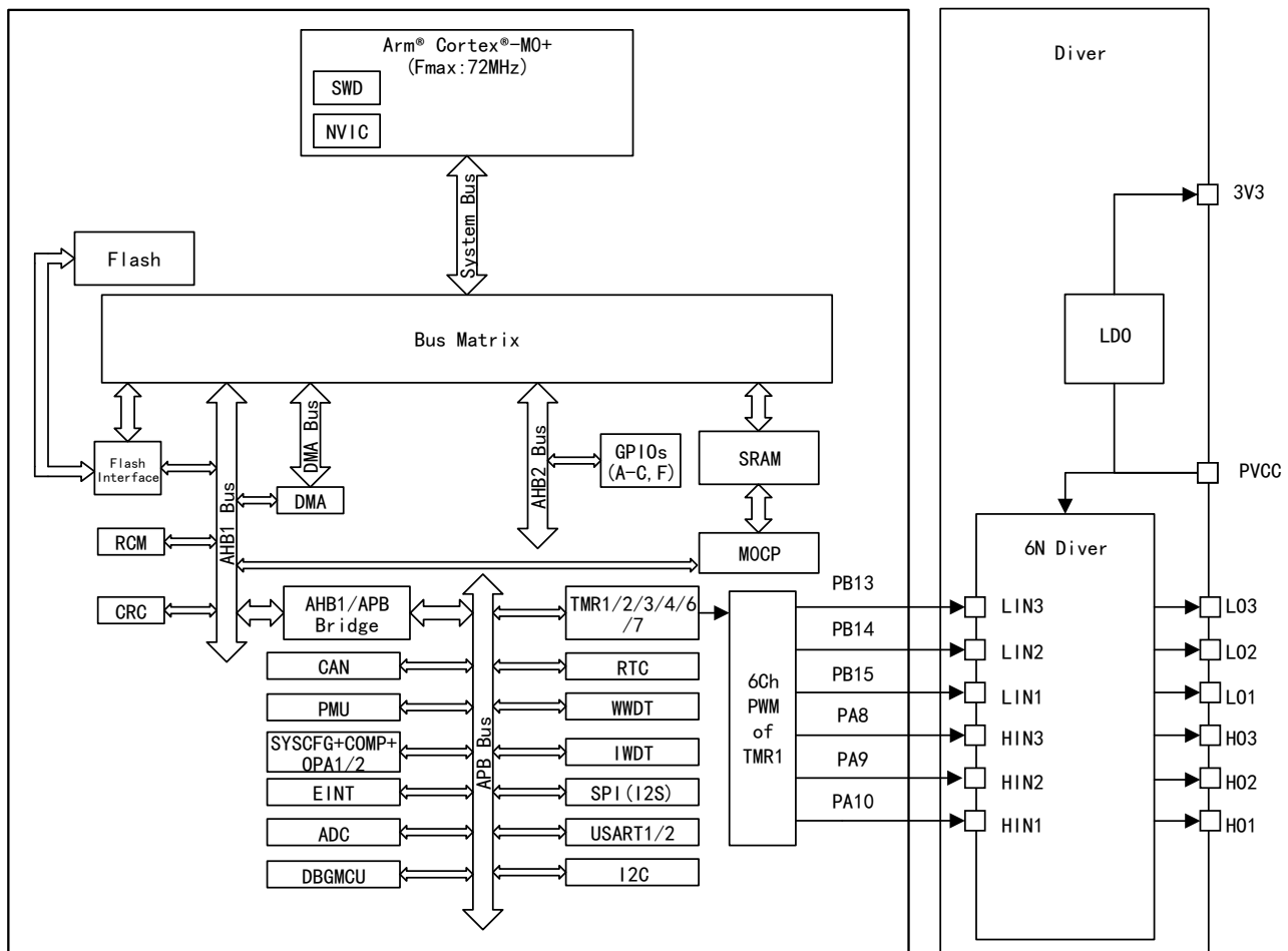
Figure 5 APM32M3514x8 System Block Diagram
